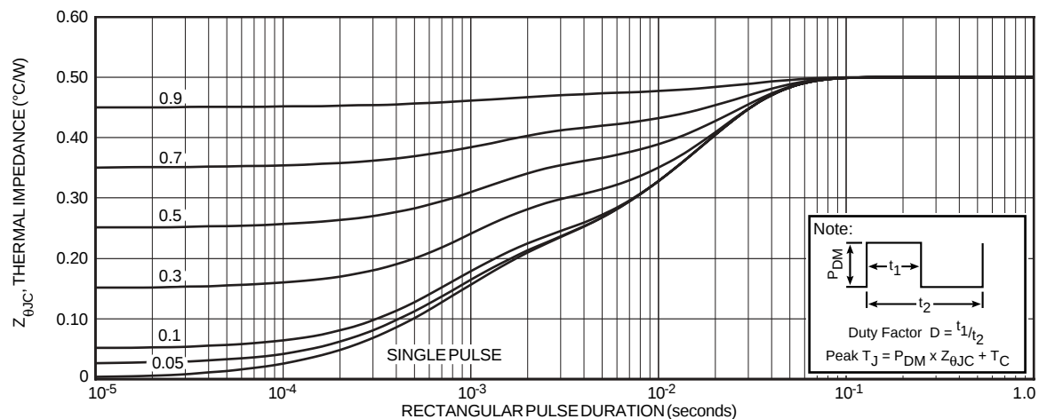
FIGURE 9a. MAXIMUM EFFECTIVE TRANSIENT THERMAL IMPEDANCE, JUNCTION-TO-CASE vs. PULSE DURATION
