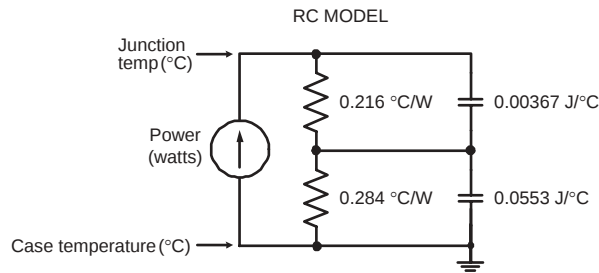
FIGURE 2, TRANSIENT THERMAL IMPEDANCE MODEL
